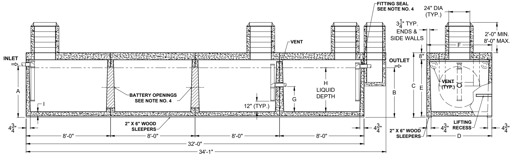
SECTION THRU "A-A"
